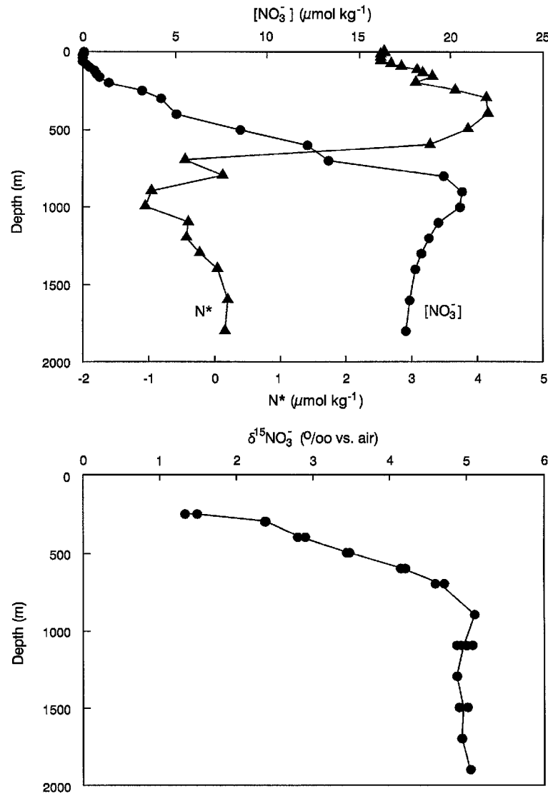
Figure 5. Depth profiles at the Bermuda Atlantic Time-series Study (BATS) station of (top) nitrate concentration and N^* (see text), and (bottom) the \delta^{15}\text{N} of nitrate. The data in (top) were collected as part of the BATS program and the data in (bottom) are from D. Sigman (unpublished results). Individual nitrogen isotope analyses are plotted as filled circles, and the trend line passes the mean value for replicate samples at each depth. The nitrate \delta^{15}\text{N} below 800 m is close to the oceanic mean value of 5‰. The ^{15}\text{N}/^{14}\text{N} decrease toward the surface requires the addition of ^{14}\text{N} -rich nitrate to the upper water column, such as would result from the nitrification of newly fixed N. The nitrate \delta^{15}\text{N} is lowest in the shallow thermocline, where the N^* data suggest that the addition of newly fixed N is greatest in proportion to the nitrate concentration.
