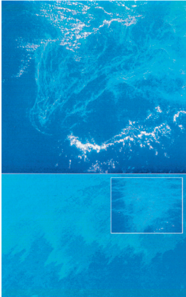
Figure 3. Trichodesmium bloom as viewed from space to the sea surface. [TOP] A massive Trichodesmium bloom in the Capricorn Channel of the southern Great Barrier Reef, Australia (near 22°50'S, 152°50'E) as viewed from the U.S. Space Shuttle flight STS-9, November 1983. This photo was taken using a hand-held 70 mm Hasselblad camera from a perspective 300 km above the Earth; the scale is approximately 1:850,000 (Reproduced from Kuchler & Jupp 1988); [BOTTOM] A massive Trichodesmium bloom in the North Pacific Subtropical Gyre (near 22°48'N, 158°11'W) as viewed from a U.S. Coast Guard C-130 aircraft (altitude 1.2 km), August 1989. The inset is a shipboard view of this same bloom from the deck of the SSP Kaimalino (photo credits: K. Louder and D. Hebel, inset).
